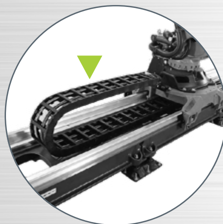
Guide Module® FLEX installs internally or externally to select robotic cable carriers for smooth wire delivery.
