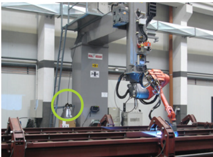
Wire Feed Assist installed in a robotic gantry application.
