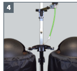
4 When wire from drum 1 runs out, the transfer arm will switch over to drum 2. Simply replace empty drum and repeat steps 1 - 3.
