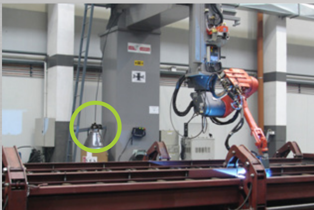
Wire Feed Assist installed in a robotic gantry application.
