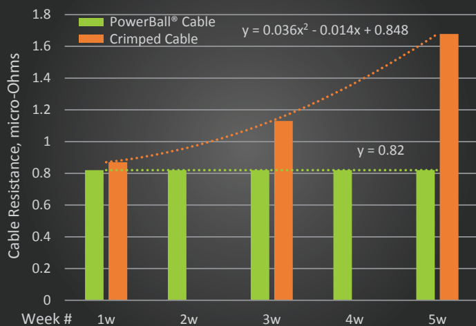
Cable Resistance Degradation Under Thermal Load
